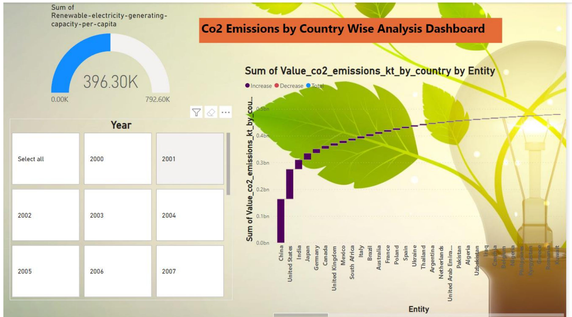
Figure 3.25 Project Dashboard 2
